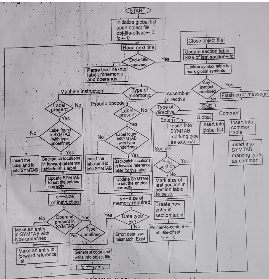
FIGURE 3.15 Single-pass assembler.
